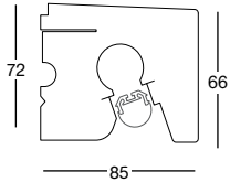
PL214 profilo lineare linear profile
