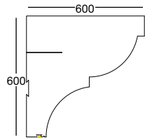
PLE711 profilo lineare linear profile
